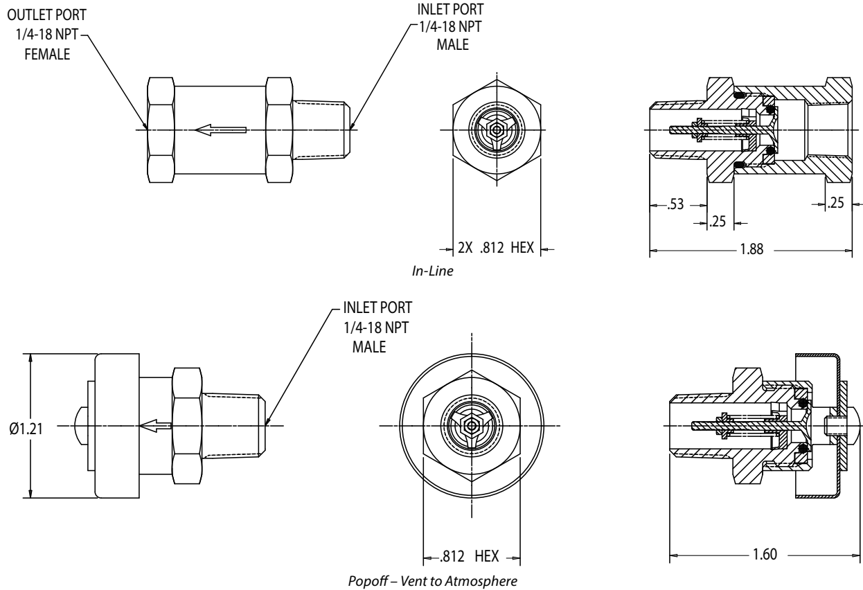
CSC L500-2MP Relief Valve (Inline) Flow Data (ESR 21625)
